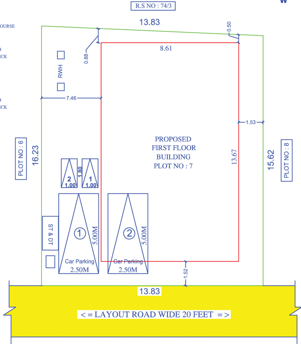
SITE PLAN
