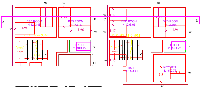
EXISTING FIRST FLOOR PLAN
