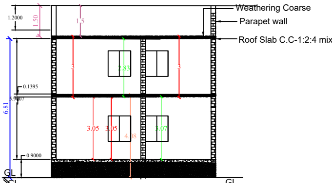
CROSS SECTION ON ABCD
