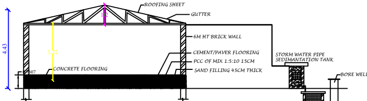
CROSS SECTION ON XX
