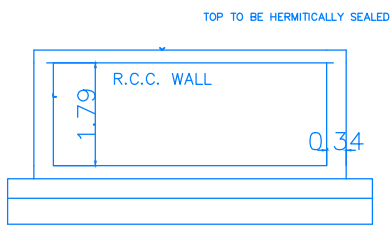
RWH_SECTION (SAMPLE) RWH_CAPACITY_L = 2000LTRS
