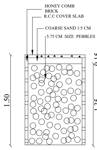
SECTION
