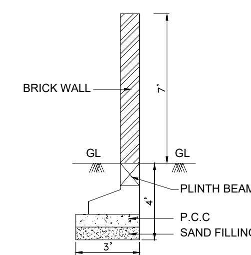
COMPOUND WALL DETAIL
