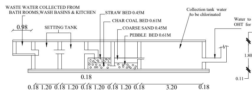
SECTION
