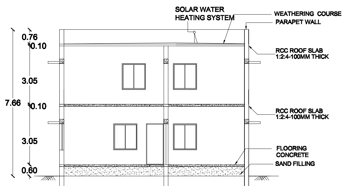
SECTION ON RM
