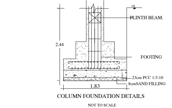
COLUMN FOUNDATION DETAILS NOT TO SCALE
