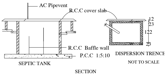
SECTION
