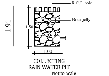
COLLECTING RAIN WATER PIT Not to Scale RW_CAPACITY_L=1000 LTRS
