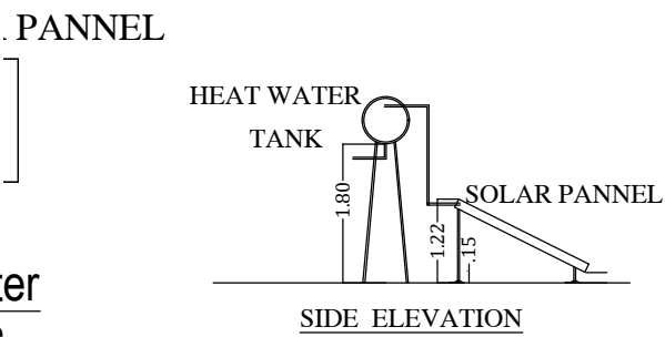
SIDE ELEVATION
