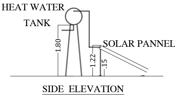
SIDE ELEVATION
