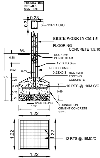
FOUNDATION DETAILS Scale: 1:50
