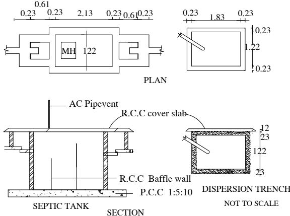
SEPTIC TANK SECTION
