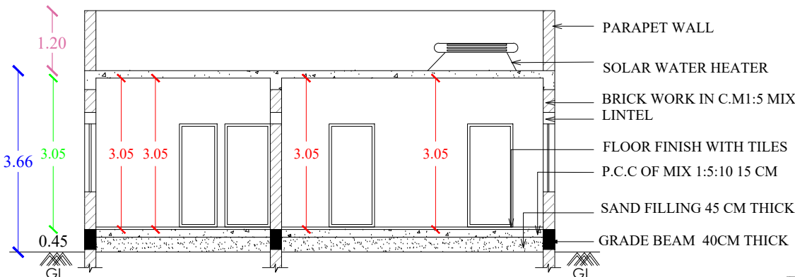
SECTION- AA1
