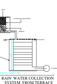
RAIN WATER COLLECTION SYSTEM FROM TERRACE
