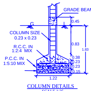
COLUMN DETAILS SCALE 1:25
