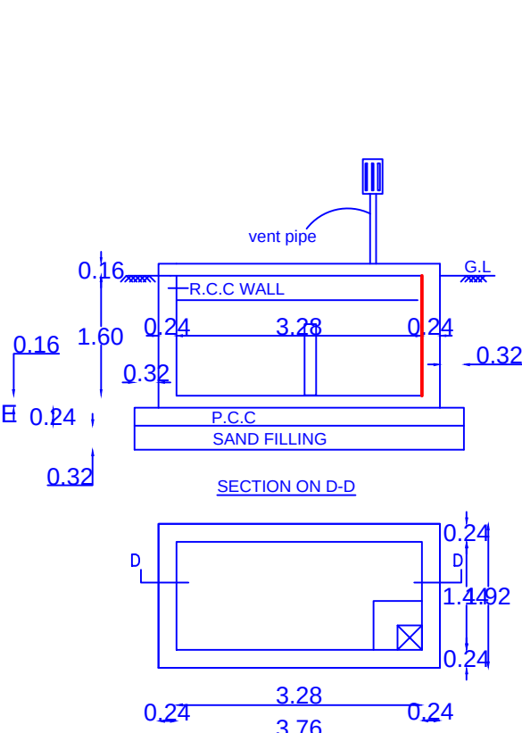
PLAN OF SEPTIC TANK
