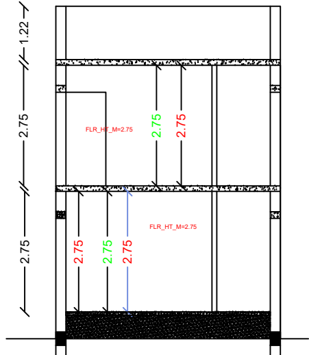
SECTION AT AB
