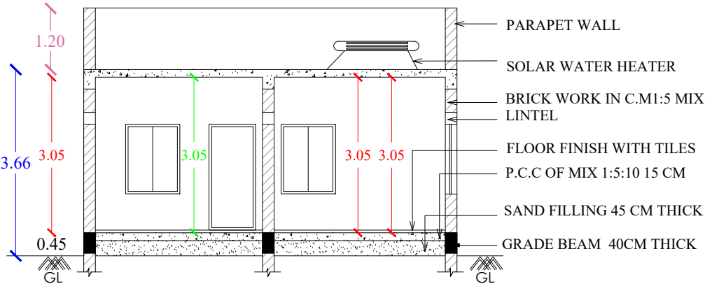
SECTION- AA1
