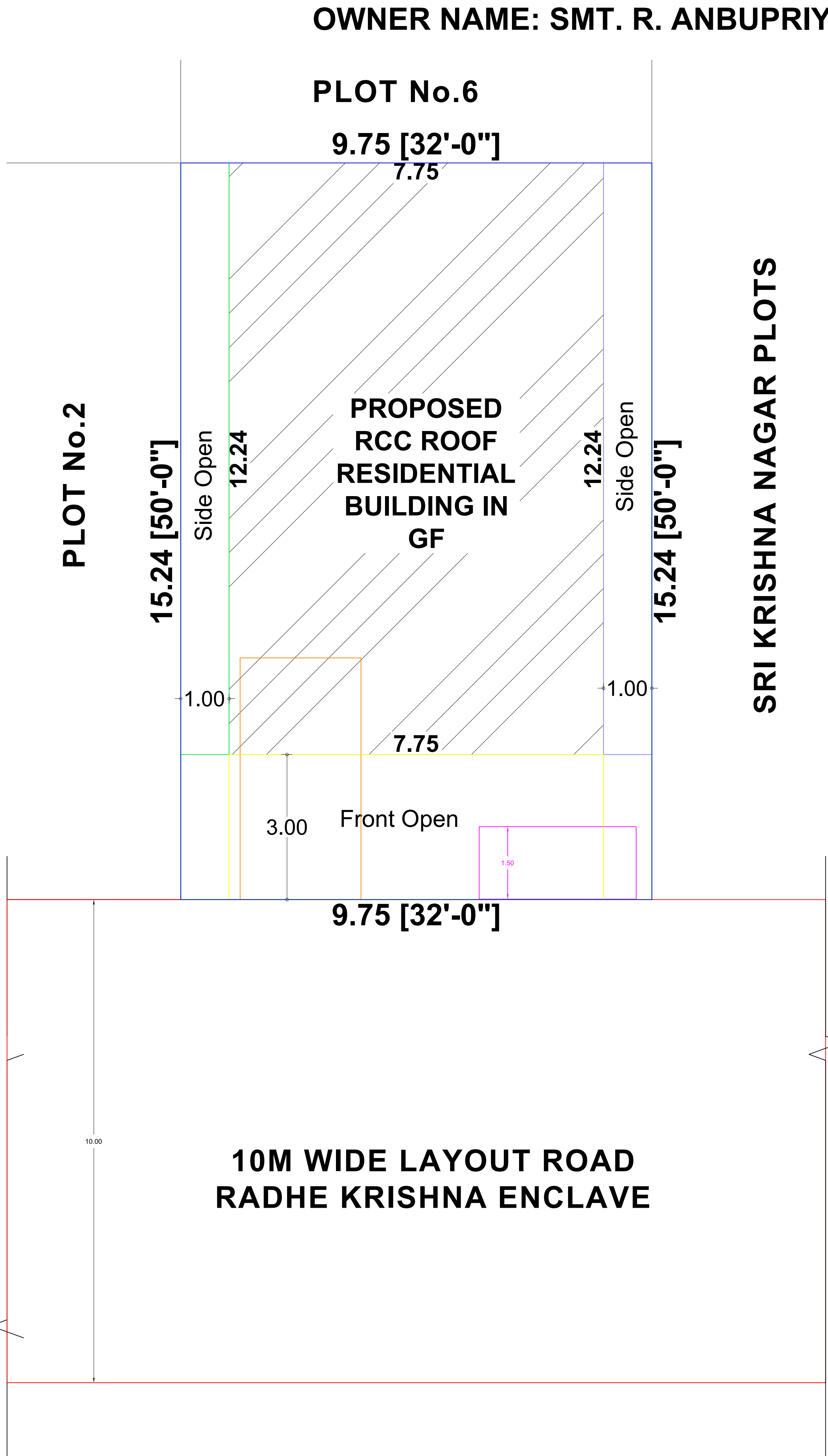
SITE PLAN [1:100]
