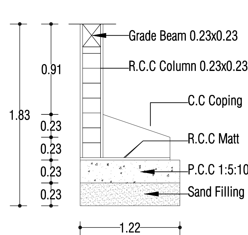
Foundation Details
