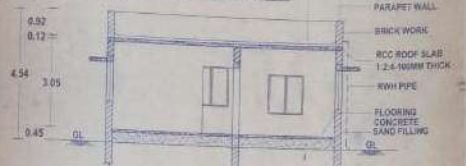
SECTION X-Y
