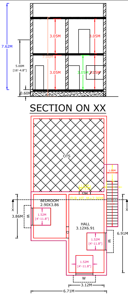
PRO.FIRST FLOOR PLAN
