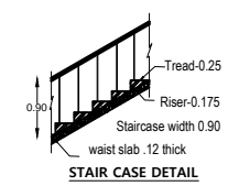
STAIR CASE DETAIL
