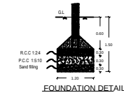
FOUNDATION DETAIL
