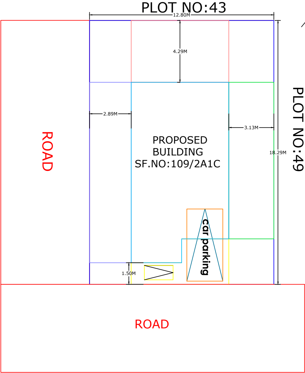
SITE PLAN
