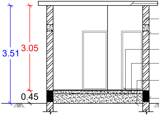
SECTION-AA1
