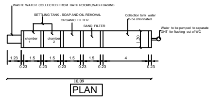
WASTE WATER RECYCLING SYSTEM
