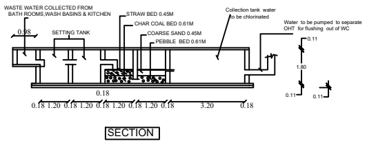
SECTION
