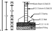
Foundation Detail
