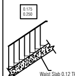
Staircase Details
