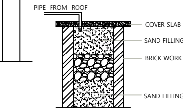
RAIN WATER HARVESTING R.W.H
