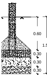
FOUNDATION DETAIL
