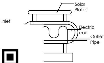
RAIN WATER HARVESTING SYSTEM
