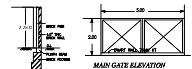
MAIN GATE ELEVATION
