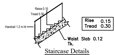
Staircase Details
