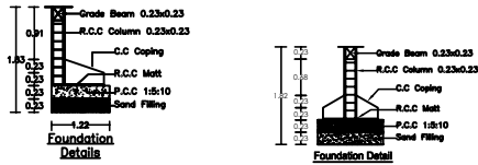
Foundation Detail
