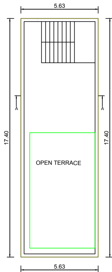
PROPOSED TERRACE FLOOR PLAN
