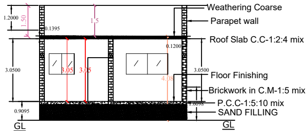
CROSS SECTION ON XX
