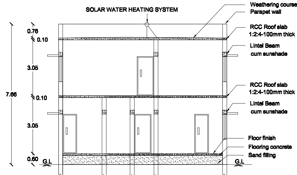
SECTION ON MK
