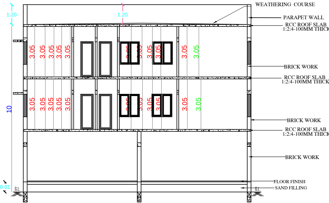
SECTION - XX
