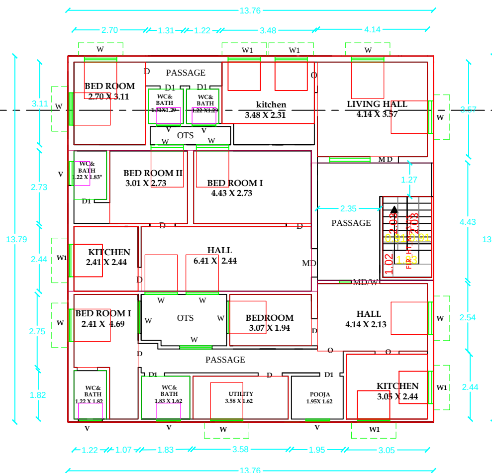
PRO. SECOND FLOOR PLAN
