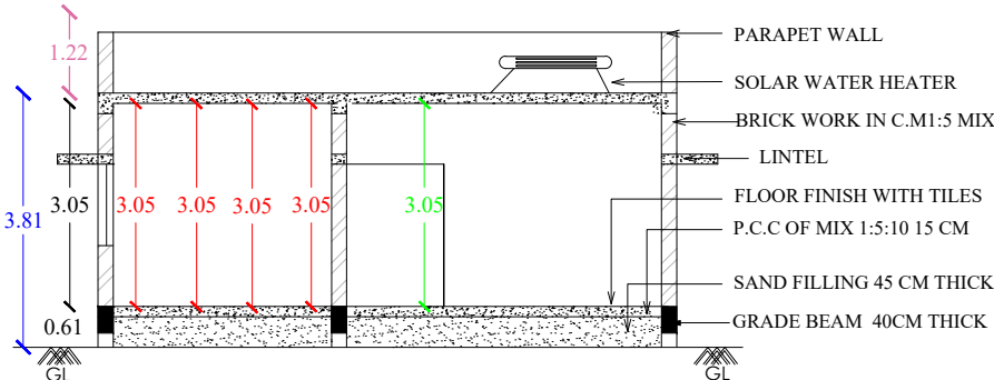
SECTION- AA1
