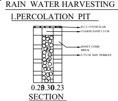
RAIN WATER HARVESTING I.PERCOLATION PIT SECTION PLAN
