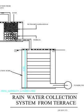
RAIN WATER COLLECTION SYSTEM FROM TERRACE
