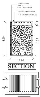
PLAN
