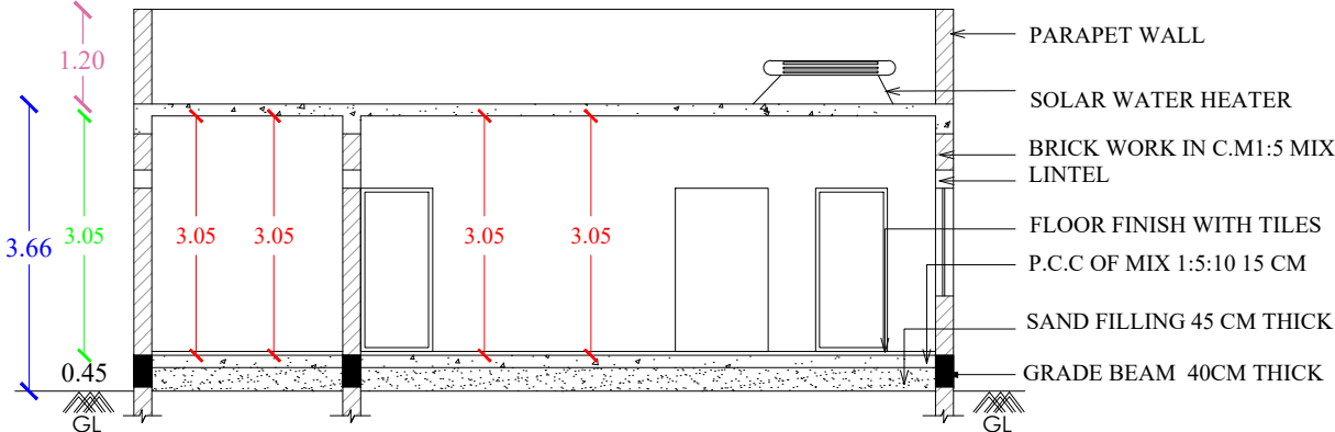
SECTION- AA1
