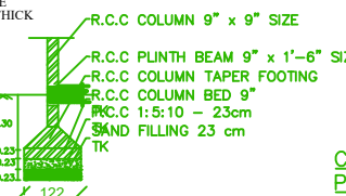
COLUMN DETAILS
