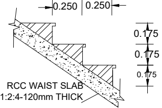
STAIR CASE STEPS SCALE 1:25
