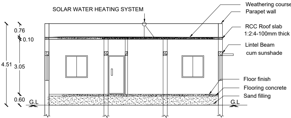
SECTION ON MK
