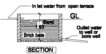
RAIN WATER HARVESTING TANK
