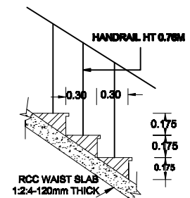
STAIR CASE STEPS SCALE 1:20
