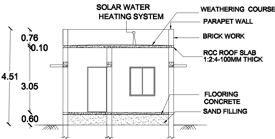
SECTION ON RM
