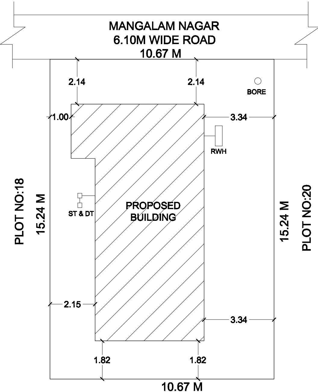
PLOT NO:25 SITE PLAN SCALE 1:100
