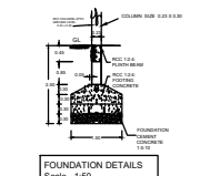
RAIN WATER HARVESTING PERCOLATION BED
