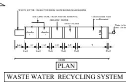
WASTE WATER RECYCLING SYSTEM
