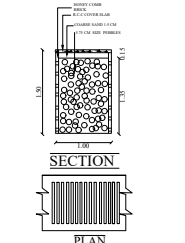
RAIN WATER HARVESTING PERCOLATION BED
