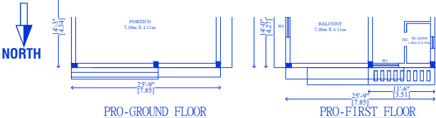
PRO-GROUND FLOOR
