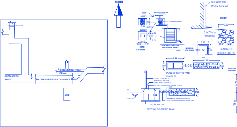
LOCATION PLAN
