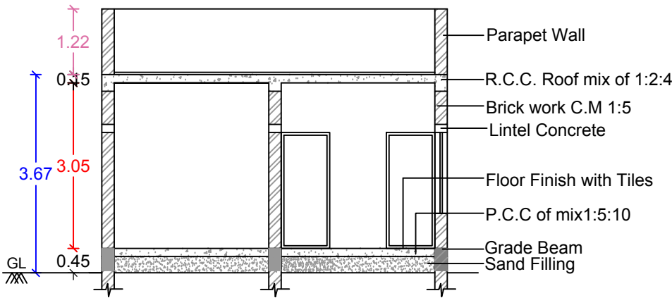
SECTION ON A-A1
