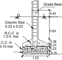
COLUMN DETAILS NOT TO SCALE
