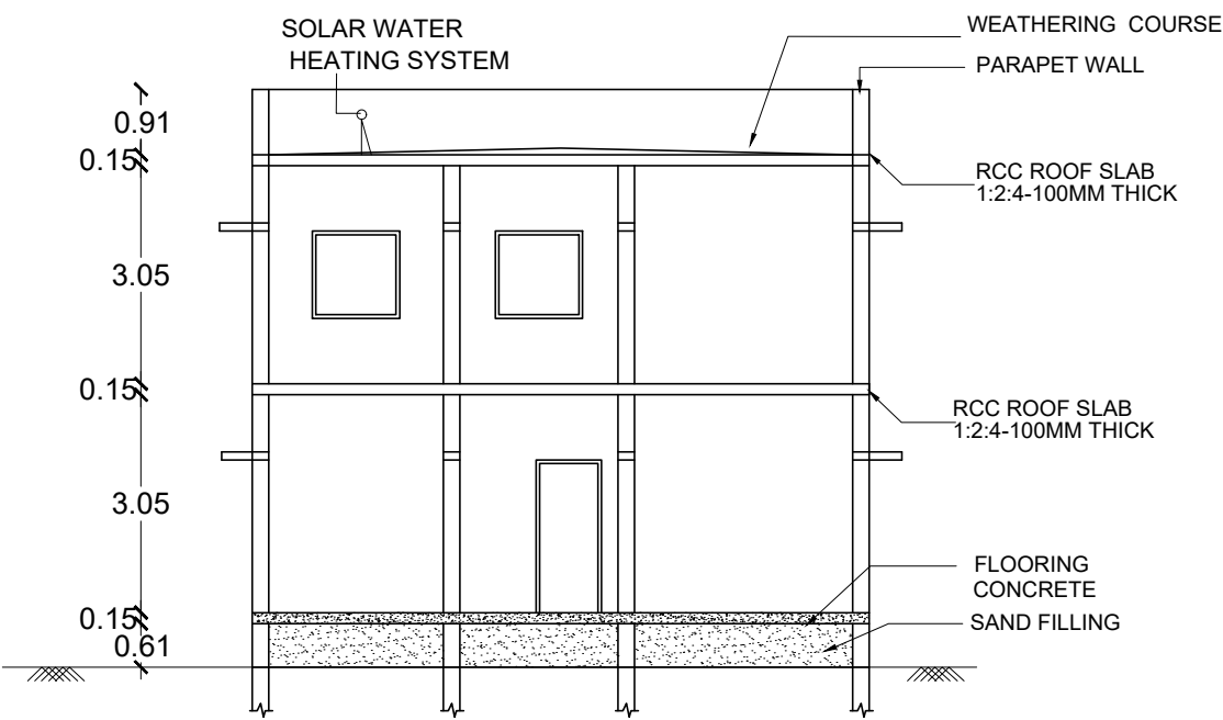
SECTION ON NP
