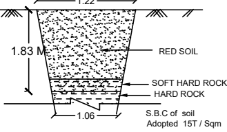
TRIAL PIT DETAILS NOT TO SCALE
