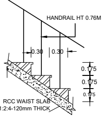
STAIR CASE STEPS SCALE 1:25
