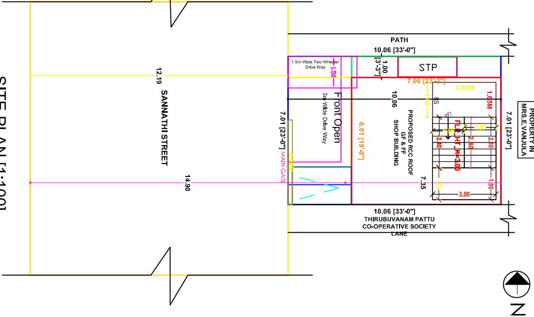
SITE PLAN [1:100]
