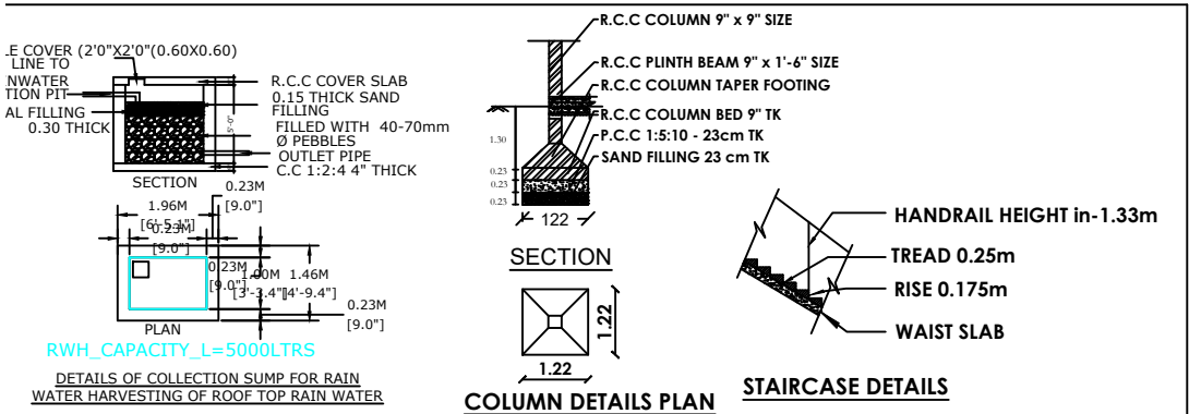
COLUMN DETAILS PLAN
