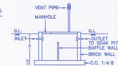
SECTION OF SEP.TANK
