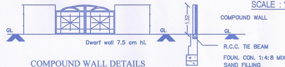
COMPOUND WALL DETAILS
