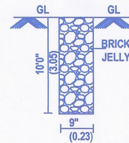
PERCULATION PIT
