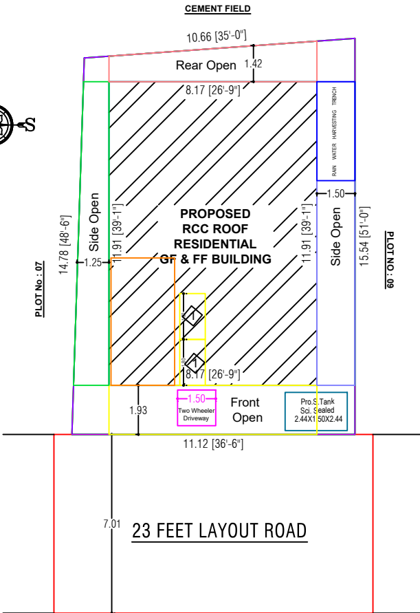
SITE PLAN [1:100]
