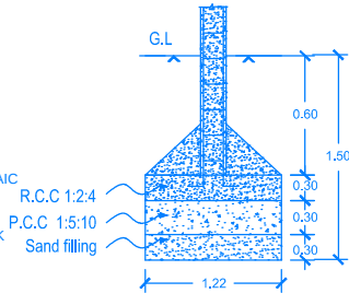
FOUNDATION DETAIL
