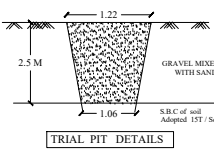
TRIAL PIT DETAILS
