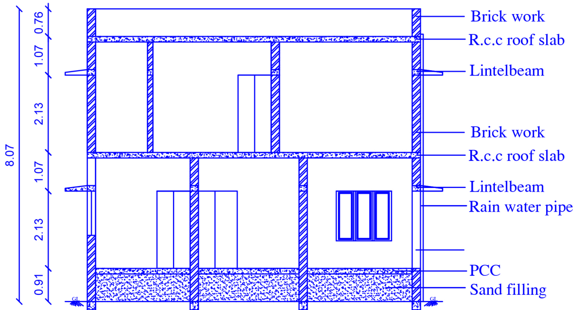
SECTION "AA"
