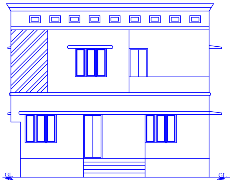
FRONT ELEVATION
