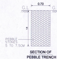
SECTION OF PEBBLE TRENCH
