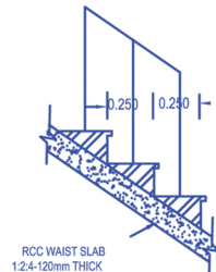
STAIR CASE DETAILS NOT TO SCALE
