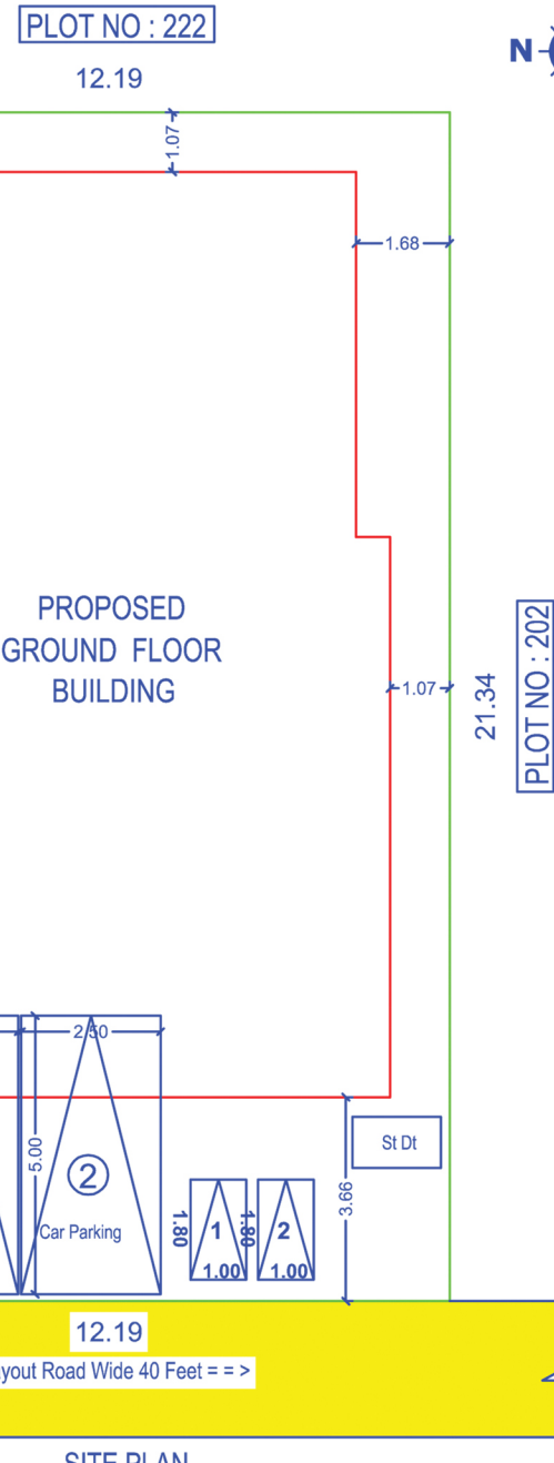
SITE PLAN
