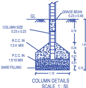
COLUMN DETAILS SCALE 1 : 50
