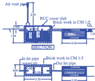
SEPTIC TANK DETAILS PLAN SCALE 1 : 200
