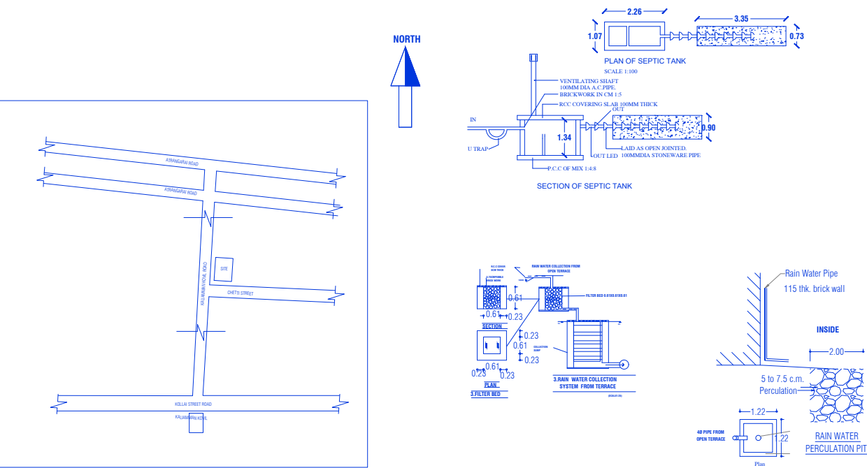
LOCATION PLAN
