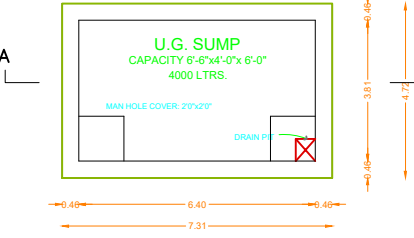
SUMP DETAIL SCALE 1"=4'0"
