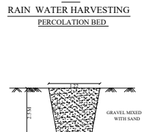
TRIAL PIT DETAILS
