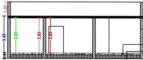
SECTION
