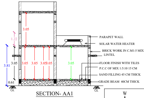
SECTION- AA1
